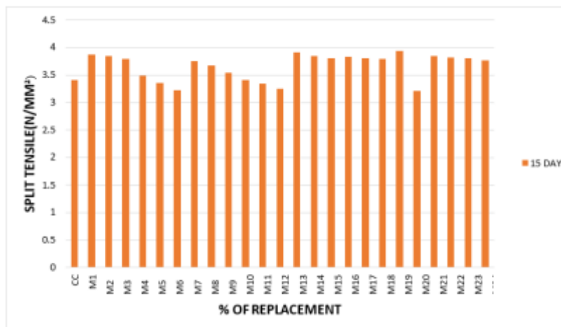
Fig 3: Split tensile test of paver blocks at 15 days
