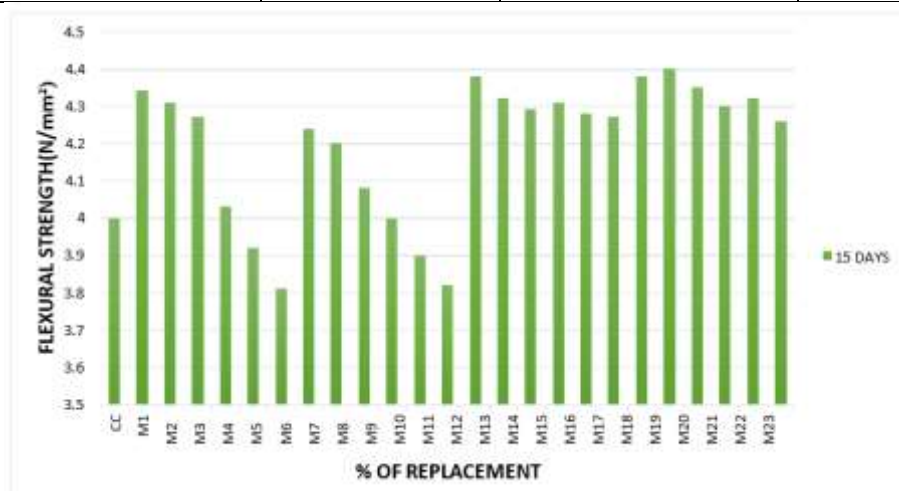
Fig 2: Flexural Strength of Paver Blocks
