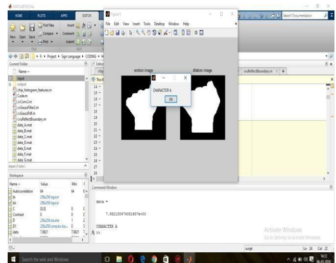
Figure 14. Output Image
