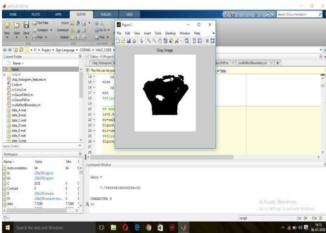
Figure 17. Gray Image
