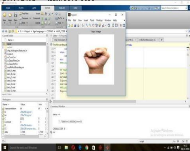
Figure 16. Input Image
