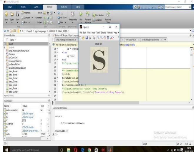
Figure 22. Output Image
