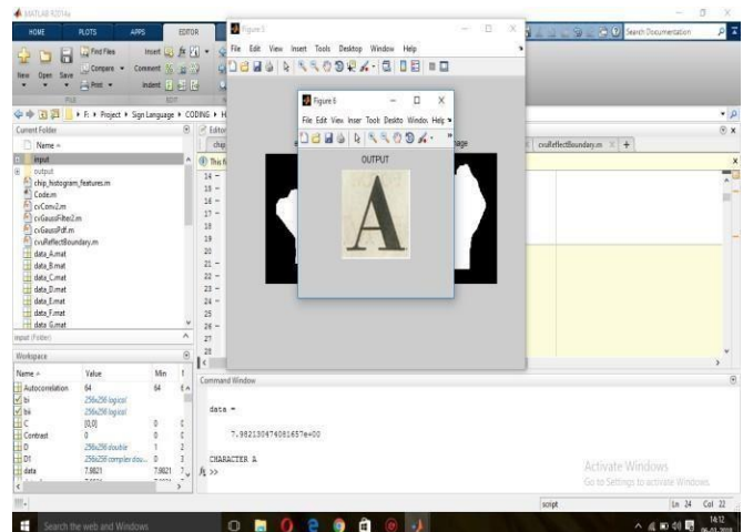
Figure 15. Output Image
