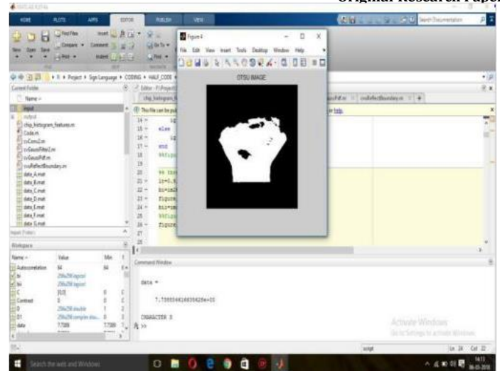
Figure 19. Otsu Image
