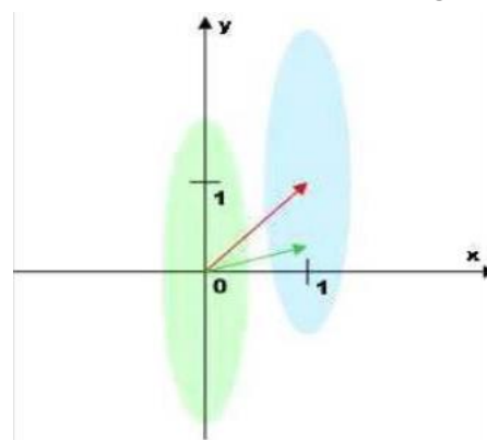
Figure 2. LDA approach
