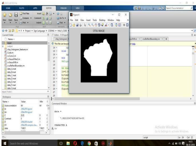
Figure 12. Otsu Image
