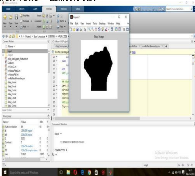
Figure 10. Gray Image
