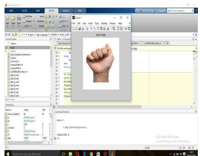
Figure 9. Input Image
