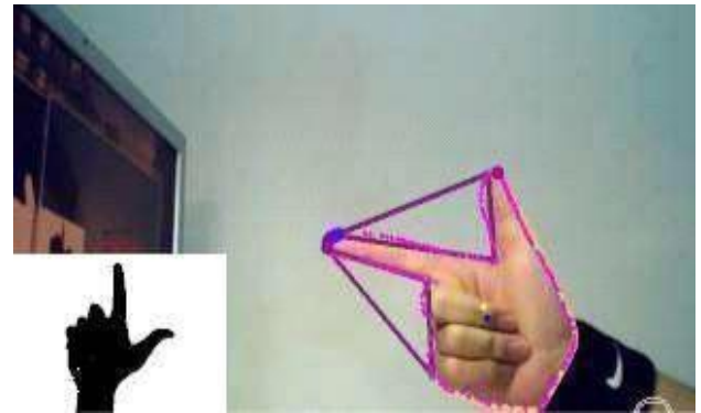
Figure 8. Dimensionality reduction
