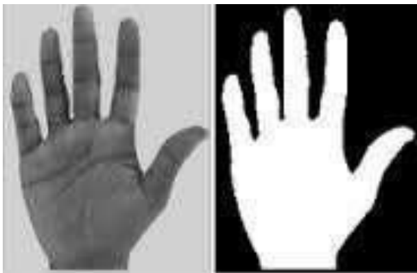
Figure 4. Segmented image
