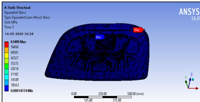
Figure 15: Equivalent stress
