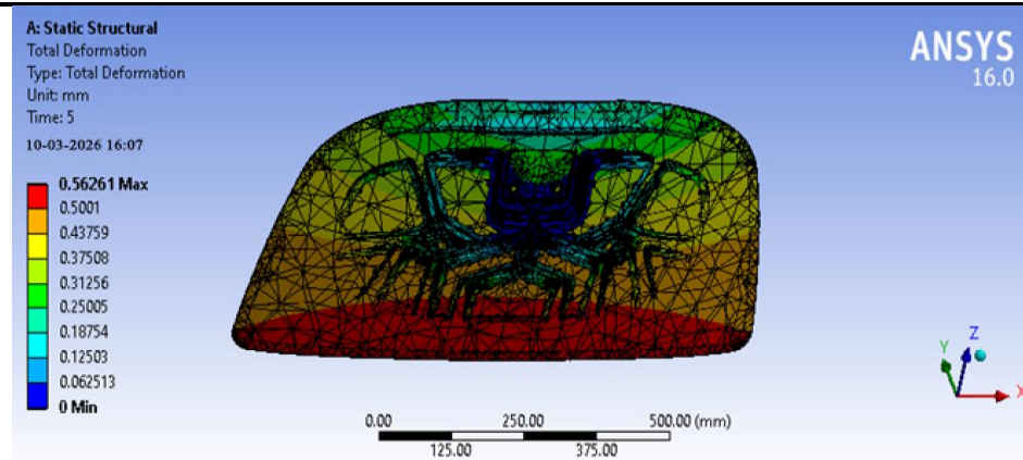
Figure 5: Total deformation
