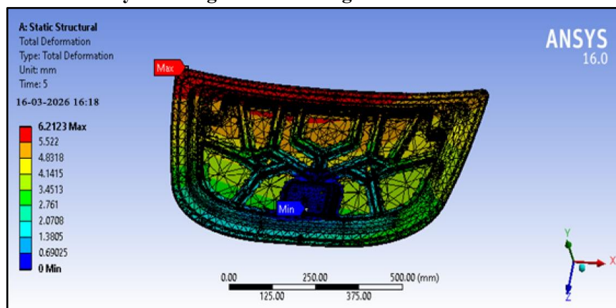
Figure 13: Total deformation
