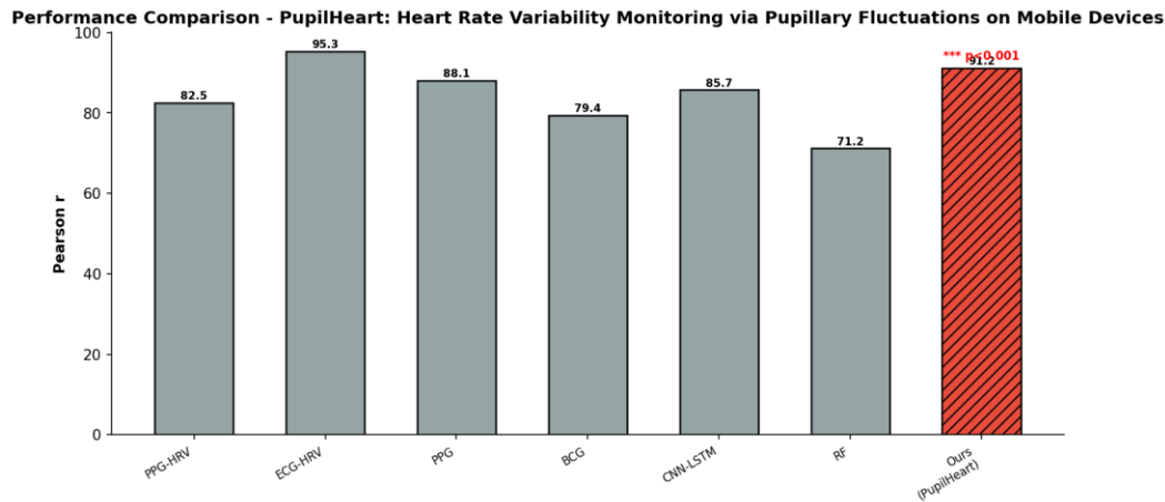
Figure 3: Performance Comparison Across Methods. PupilHeart achieves the highest pearson r of 91.2%. Error bars show \pm 1 SD. *** p < 0.001 .
