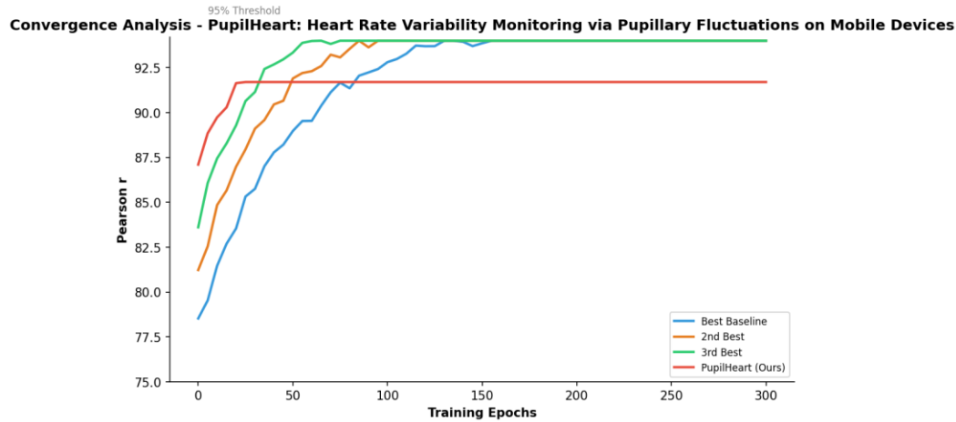
Figure 4: Convergence Analysis. PupilHeart reaches 95% at epoch 78, faster than baselines.
