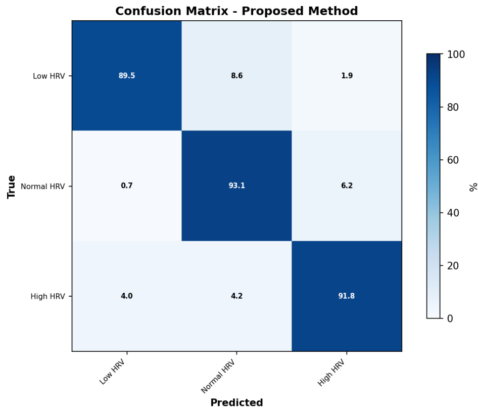
Figure 5: Confusion Matrix for PupilHeart on the Test Set. Diagonal values represent correct classification rates.
