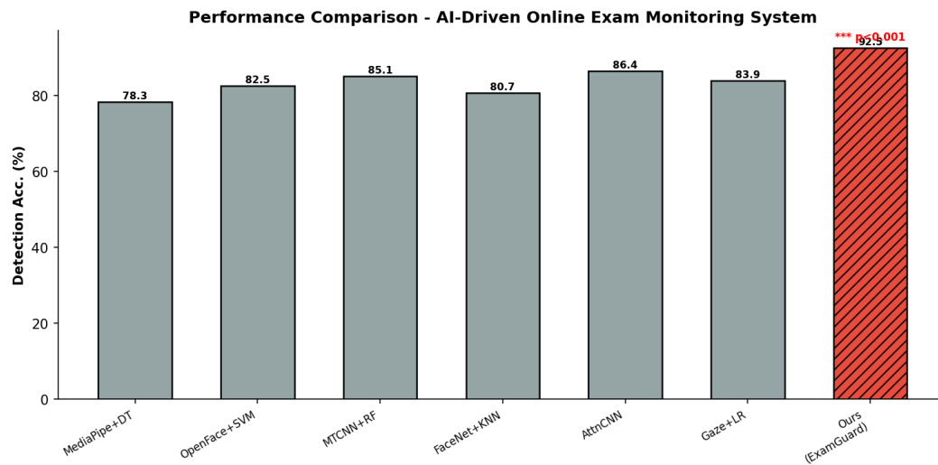
Figure 3: Performance Comparison Across Methods. ExamGuard achieves the highest detection acc. (%) of 92.5%. Error bars show \pm 1 SD. *** p < 0.001 .
