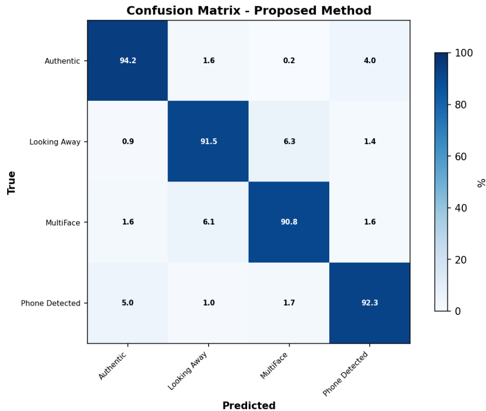
Figure 5: Confusion Matrix for ExamGuard on the Test Set. Diagonal values represent correct classification rates.
