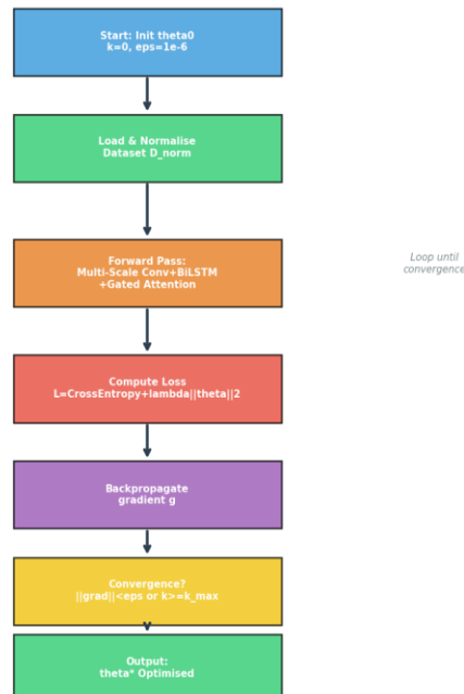
Figure 2: Algorithmic Flowchart of the ExamGuard Training Procedure. Step numbers correspond to Algorithm 1.
