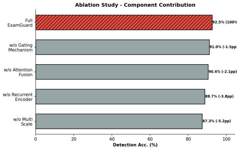
Figure 6: Ablation Study - Component Contribution. The recurrent encoder provides the largest single contribution.
