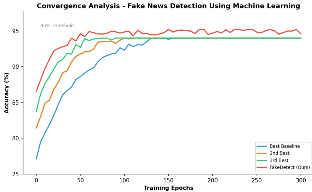
Figure 4: Convergence Analysis. FakeDetect reaches 95% at epoch 55, faster than baselines.
