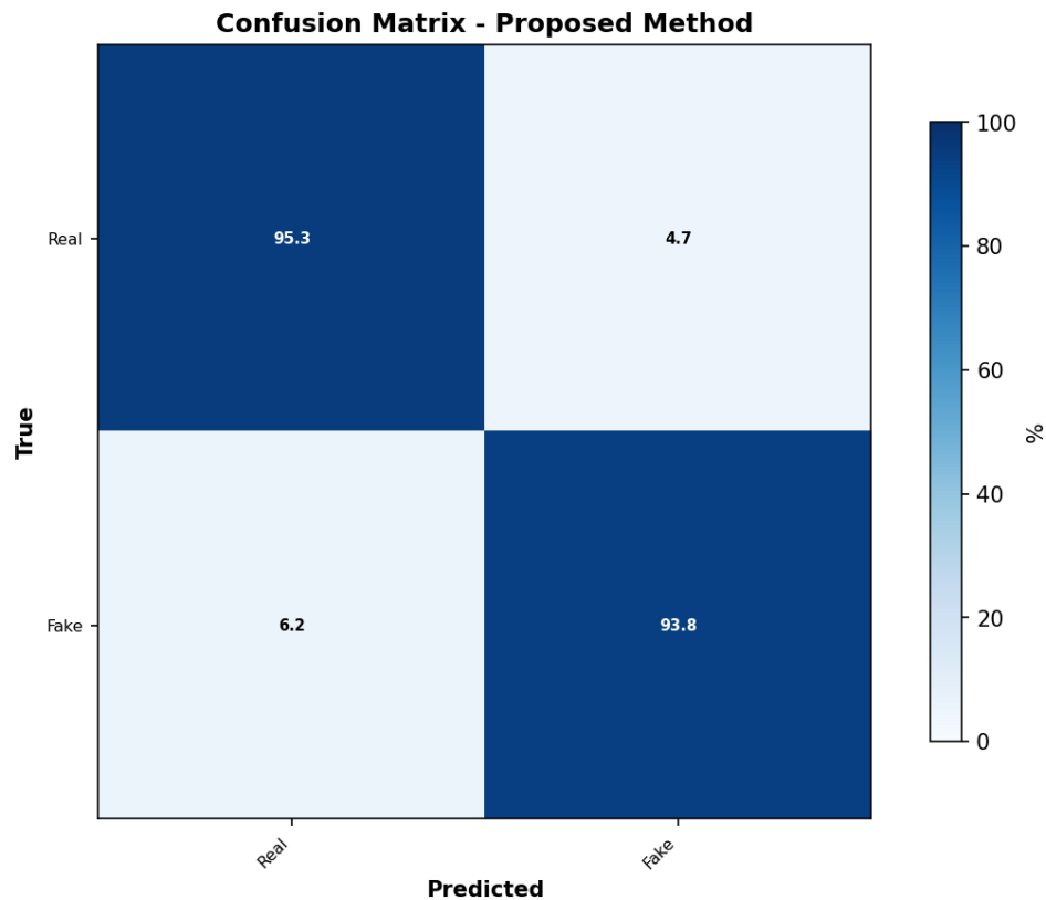
Figure 5: Confusion Matrix for FakeDetect on the Test Set. Diagonal values represent correct classification rates.
