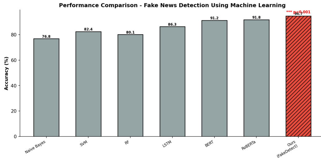
Figure 3: Performance Comparison Across Methods. FakeDetect achieves the highest accuracy (%) of 94.7%. Error bars show \pm 1 SD. *** p < 0.001 .
