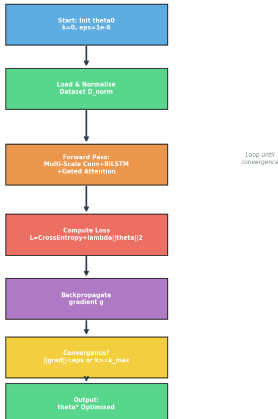
Figure 2: Algorithmic Flowchart of the FakeDetect Training Procedure. Step numbers correspond to Algorithm 1.
