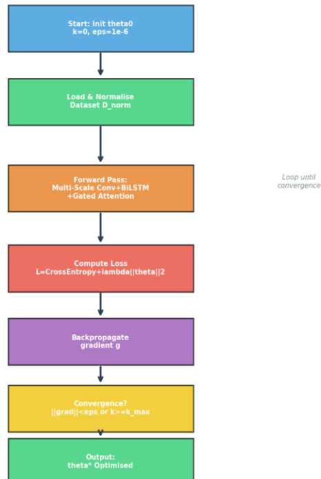
Figure 2: Algorithmic Flowchart of the LogoGuard Training Procedure. Step numbers correspond to Algorithm 1.
