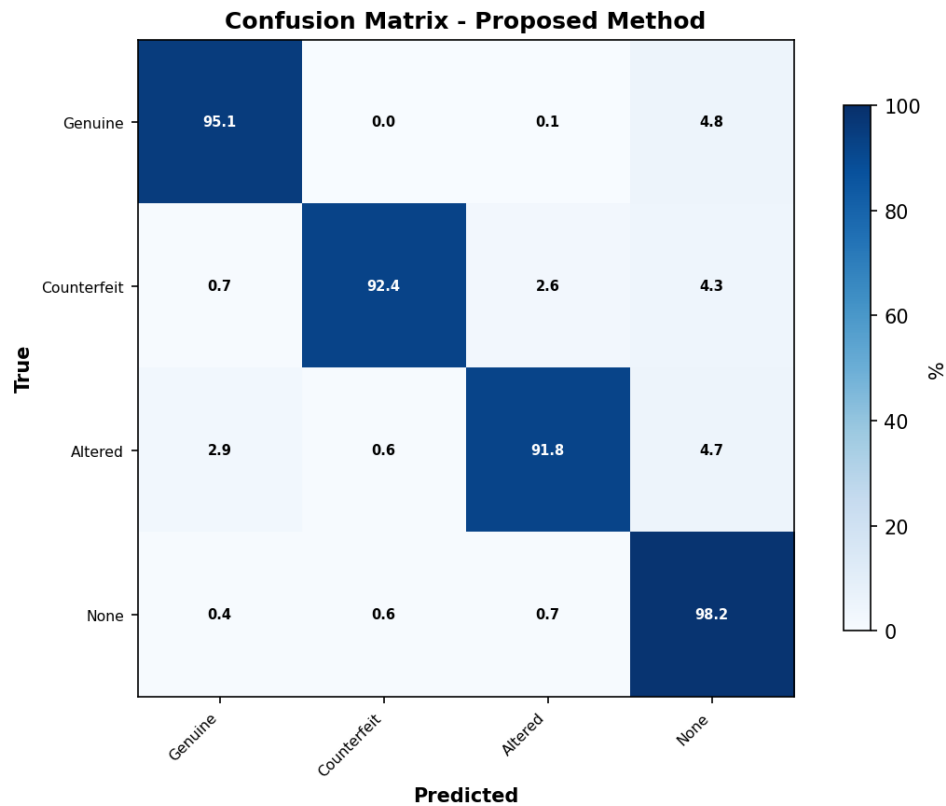
Figure 5: Confusion Matrix for LogoGuard on the Test Set. Diagonal values represent correct classification rates.
