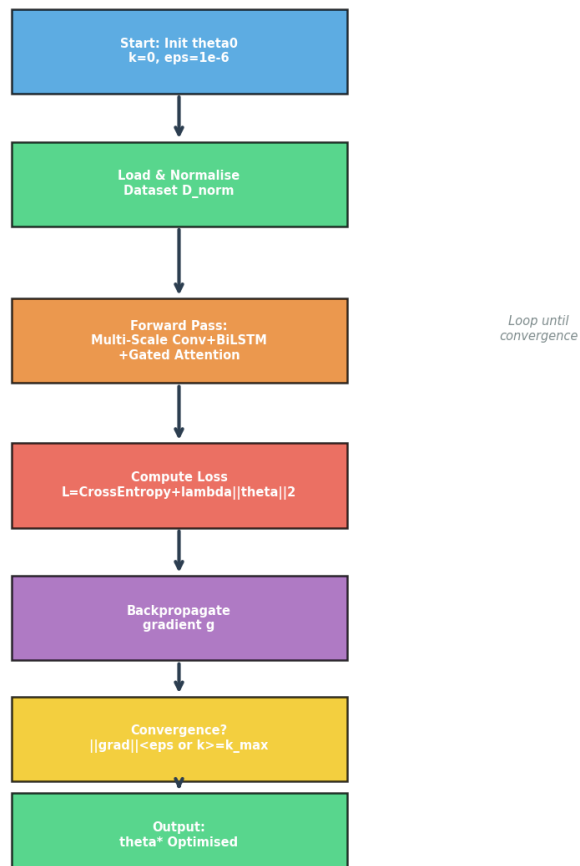
Figure 2: Algorithmic Flowchart of the FingerLock Training Procedure. Step numbers correspond to Algorithm 1.
