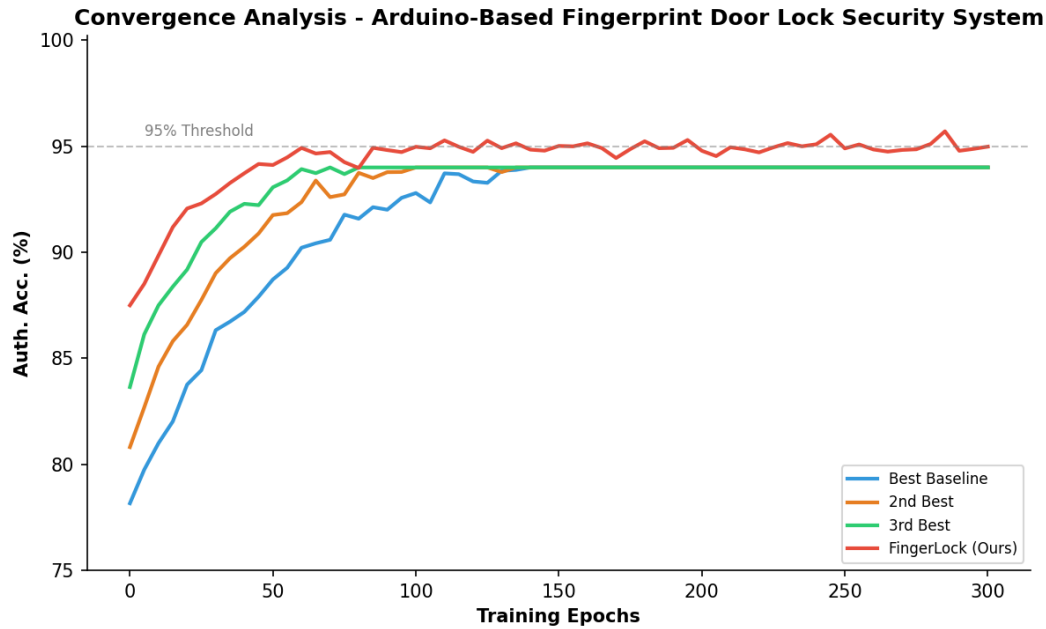
Figure 4: Convergence Analysis. FingerLock reaches 95% at epoch 65, faster than baselines.
