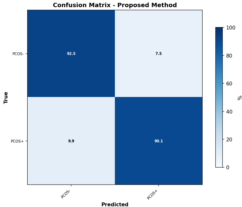
Figure 5: Confusion Matrix for PCOSense on the Test Set. Diagonal values represent correct classification rates.
