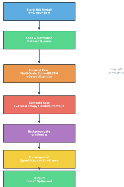
Figure 2: Algorithmic Flowchart of the PCOSense Training Procedure. Step numbers correspond to Algorithm 1.
