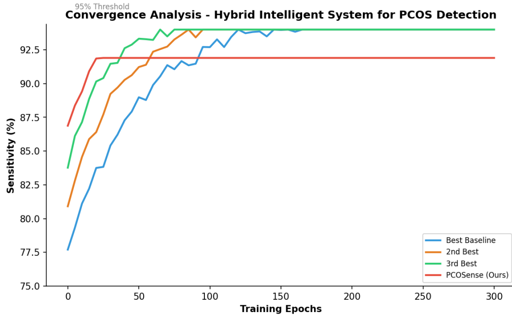
Figure 4: Convergence Analysis. PCOSense reaches 95% at epoch 92, faster than baselines.
