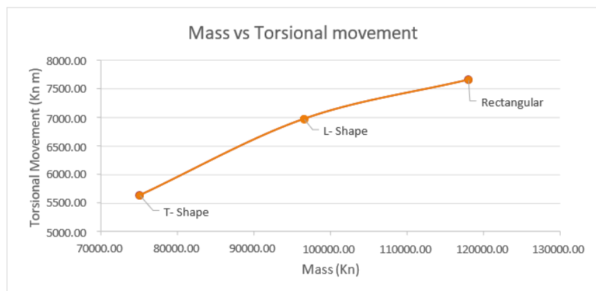
Figure 6: Mass v/s Torsional Movement
