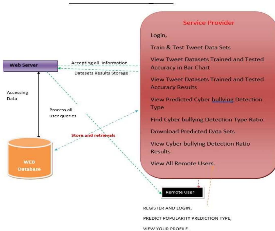
Fig 1. Architecture Diagram
