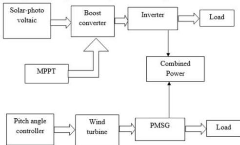
Fig 1. Block diagram of hybrid system
