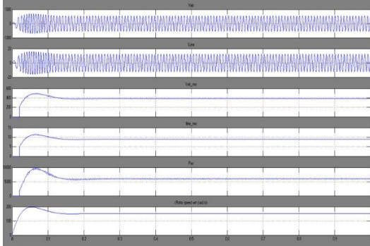
Fig. 14 Voltage, current and power of PMSG
