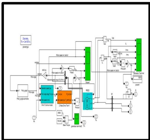
Fig. 12 Simulink block of wind energy conversion system
