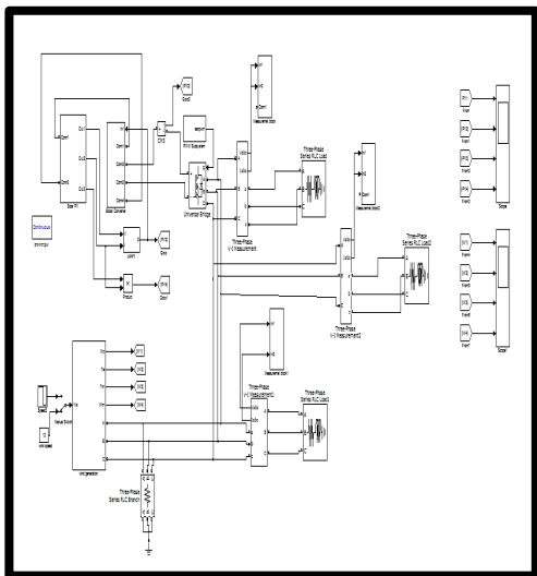
Fig. 15 Simulink block of hybrid system The simulink block of the solar photo-voltaic and permanent magnet synchronous generator based wind hybrid system has been shown in Fig: 5.10. Here, the solar energy
