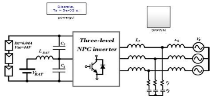
Fig. 4. Block diagram of the simulated system.
