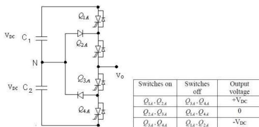
Fig. 1(b) Phase A of a 3 level inverter Table 1 Switching pattern of a phase A of 3 level inverter
