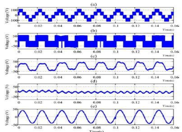
Fig 7 Simulated inverter waveforms. (a) V_{ab} -Phase to phase inverter voltage. Fig (b) V_{ao} -Inverter phase voltage reference to midpoint. (c) Filtered V_{on} -Filtered inverter phase voltage reference to midpoint. (d) Filtered V_{on} -Filtered midpoint voltage reference to neutral. (e) Filtered V_{an} -Filtered phase voltage reference to neutral.
