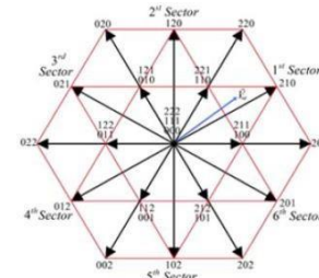
Fig. 2 Space vector diagram for the three-level diode clamped inverter
