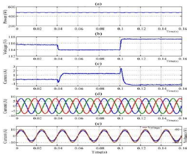
Fig 8 Simulated results for the second scenario. (a) Active power injected to the grid. (b) PV module DC voltage. (c) Battery currents. (d) Grid side currents. (e) Grid side Phase (a) voltage and its current.
