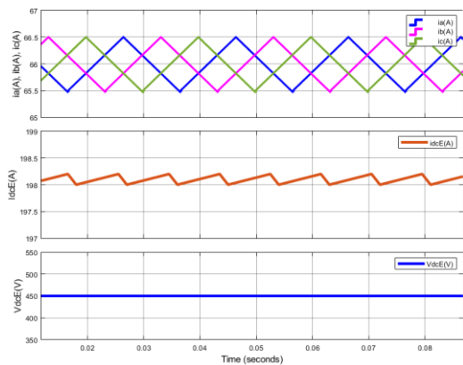
Fig 3. Simulation results: High frequency dc currents of three legs of interleaved dc-dc converter for 1.6C charging rate of EV battery ( i_a , i_b and i_c ) (A) (top
