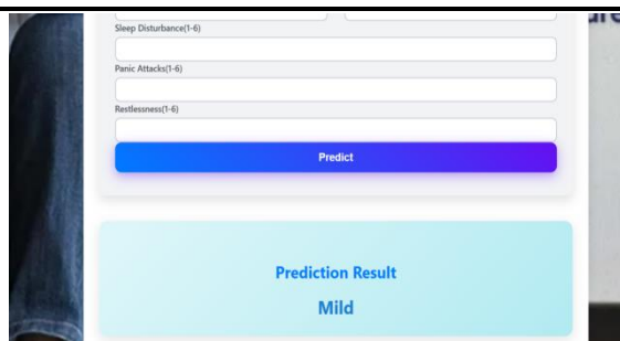
Fig 6.7 output
