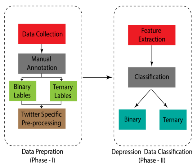
Fig 5.1: System Architecture
