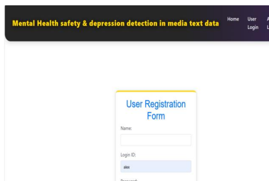
Fig 6.3 User Registratation
